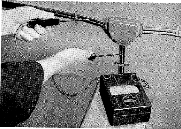
Figure 19 Measuring earth-continuity across a junction box
