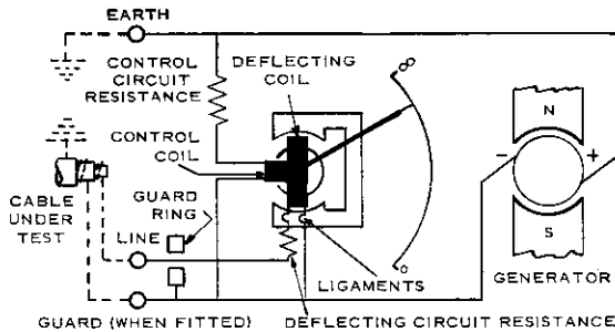
Figure 30 Series 2 instrument arranged for insulation test
