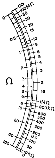
Figure 26 Series 2 (500v.)
